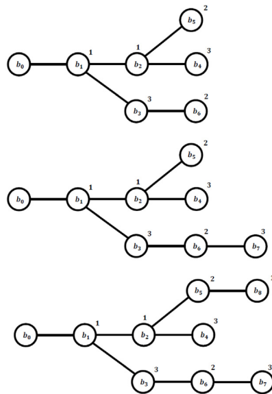
Fig. 2. Blockchain construction.
